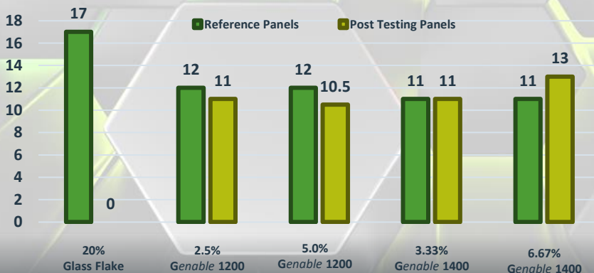
Pencil Hardness Retention
